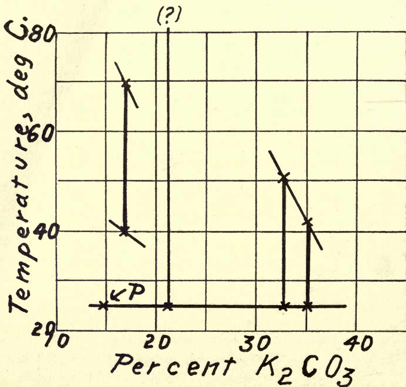
Figure 14. Upper and Lower Critical Solution Temperatures in the System: Potassium Carbonate, Ethyl Alcohol, Water.
